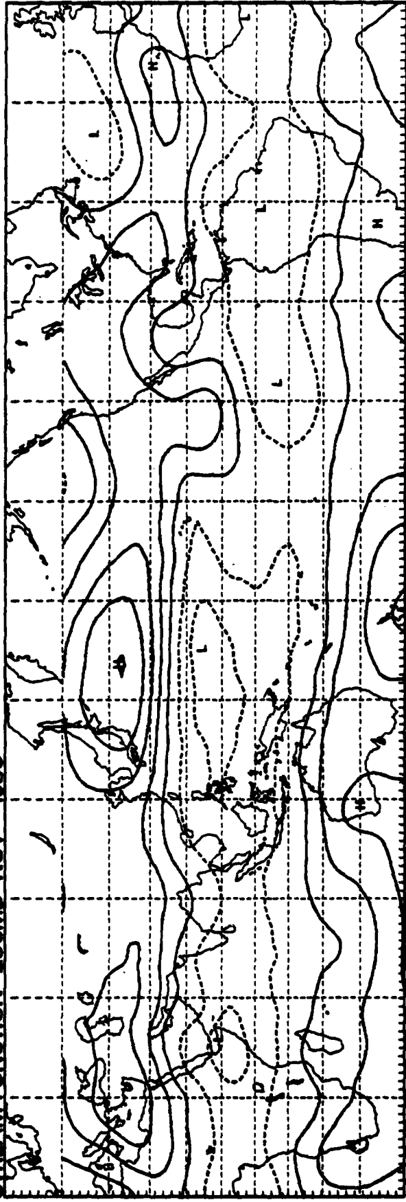
STREAM FUNCTION 200MB NOV 1980
